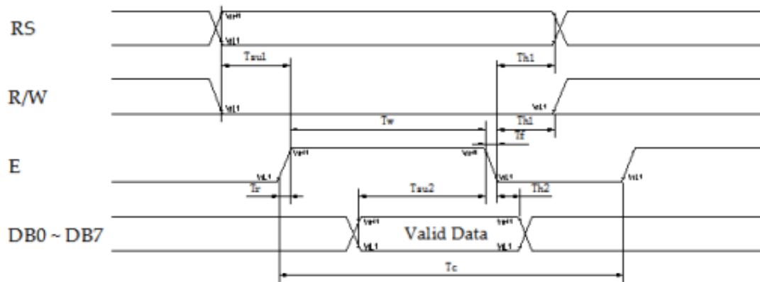
Figure 6. Write Mode Timing Diagram
